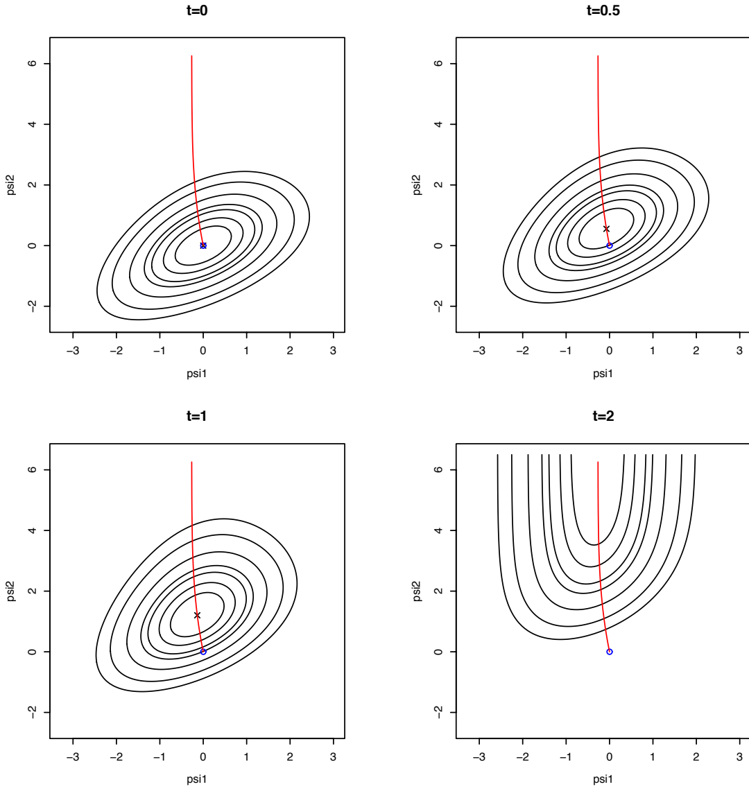
Figure 3: The tilted log-likelihood function, (4), used in (10), and the (red) curve in the parameter space traced by the maximum likelihood estimate as \mathbf{s}(t) varies along \mathcal{L}^* , for the data and model of Table 1. Each contour plot shows a point on this curve for the value of t indicated above it; the corresponding 2 \times 3 tables are in the right column of Figure 1. The maximum likelihood estimate \hat{\boldsymbol{\psi}}\{\mathbf{s}(t)\} is marked with \times , and \hat{\boldsymbol{\psi}}\{\mathbf{s}(0)\} with \circ . The lower left plot corresponds to the observed table, and the left panel of Figure 2.
