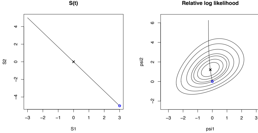
Figure 2: The line \mathcal{L}^* for testing \boldsymbol{\psi} = \mathbf{0} , using the data of Table 1. In the plane \mathcal{L}_0 on the left, the axes show the two components of \mathbf{s}_1 , as \mathbf{s}_2 = 0 on \mathcal{L}_0 . The line \mathcal{L}^* joins the (first two) components of \mathbf{s}_\psi ( \circ ) and of \mathbf{s}^0 ( \times ); see (7). In the right panel, the observed profile log-likelihood contours are plotted in (\psi_1, \psi_2) ; the constrained maximum likelihood estimate under H_\psi , and the full maximum likelihood estimate are marked with the same symbols as in the left panel. The curve in the right panel is the mapping of \mathcal{L}^0 to the parameter space.
